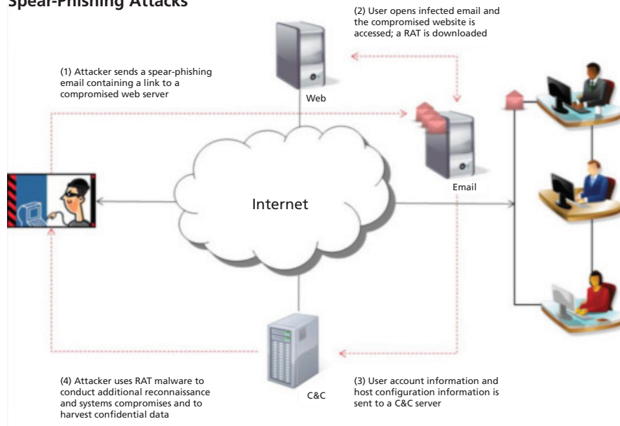
Figure 3. Spear-phishing attacks.
