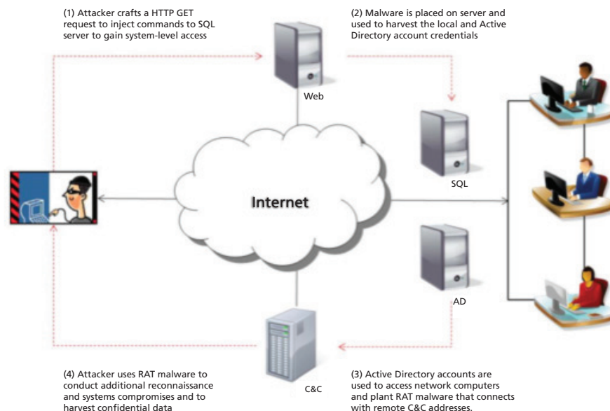
Figure 2. SQL-injection attacks.
